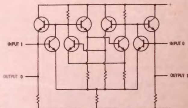
Fig. 6 R-S flipflop, essentially an astable multivibrator.
