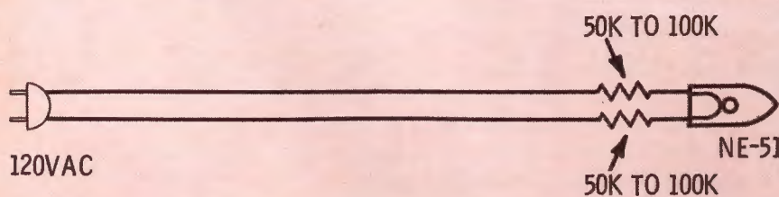
Fig. 4 The RF sniffer. The resistors should be of such value that the neon lamp barely lights.
